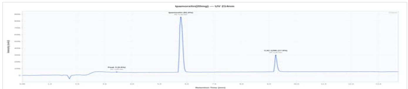
CJC-1295 / Ipamorelin 20mg - FO309: UV Chromatogram
